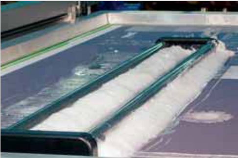
Twin roll rod system for high penetration on heavy fabrics.
