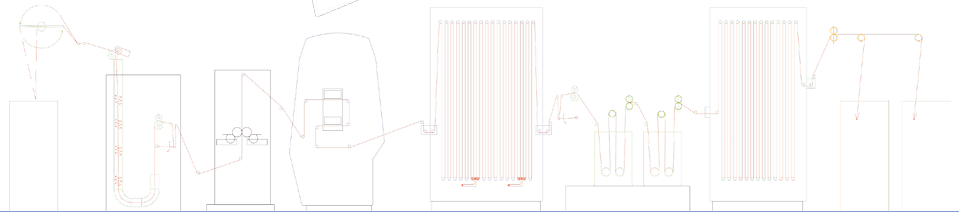
de-tangler positive in-feed section pre-treatment COLARIS-NF steamer thermosol washing boxes dryer let-off section
