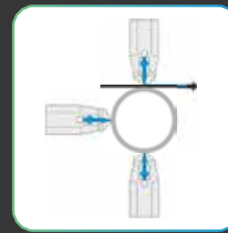
MAGNOJET direct application over-roll
