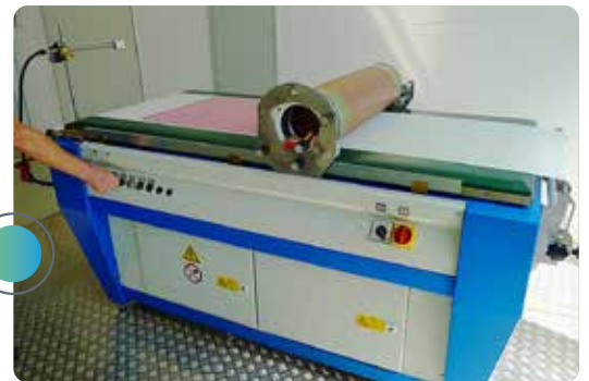
LABORATORY TABLE ROTARY SCREEN STRIKE-OFF
